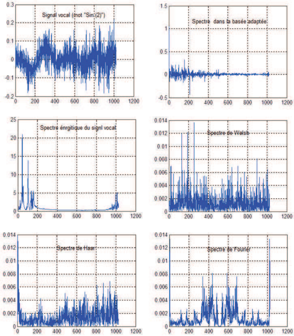
Figure 4 : Projection du signal vocal (fragment du mot \varnothing \xi / \ll \text{Sin} \gg - 2 )
